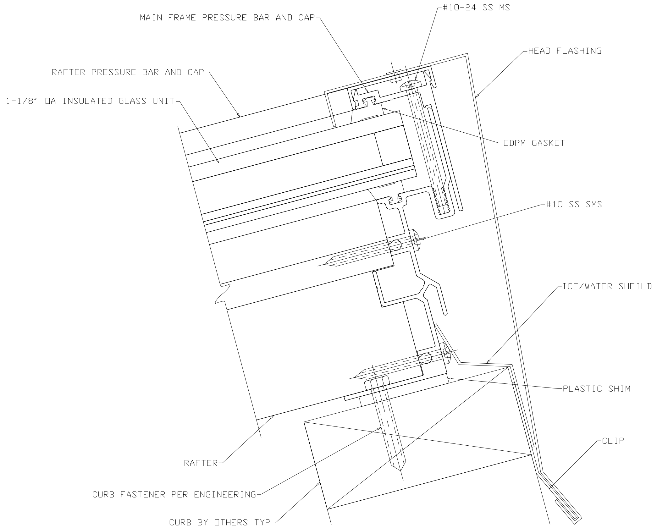
3 HEAD SECTION SCALE 1' - 0" = 1' - 0"
