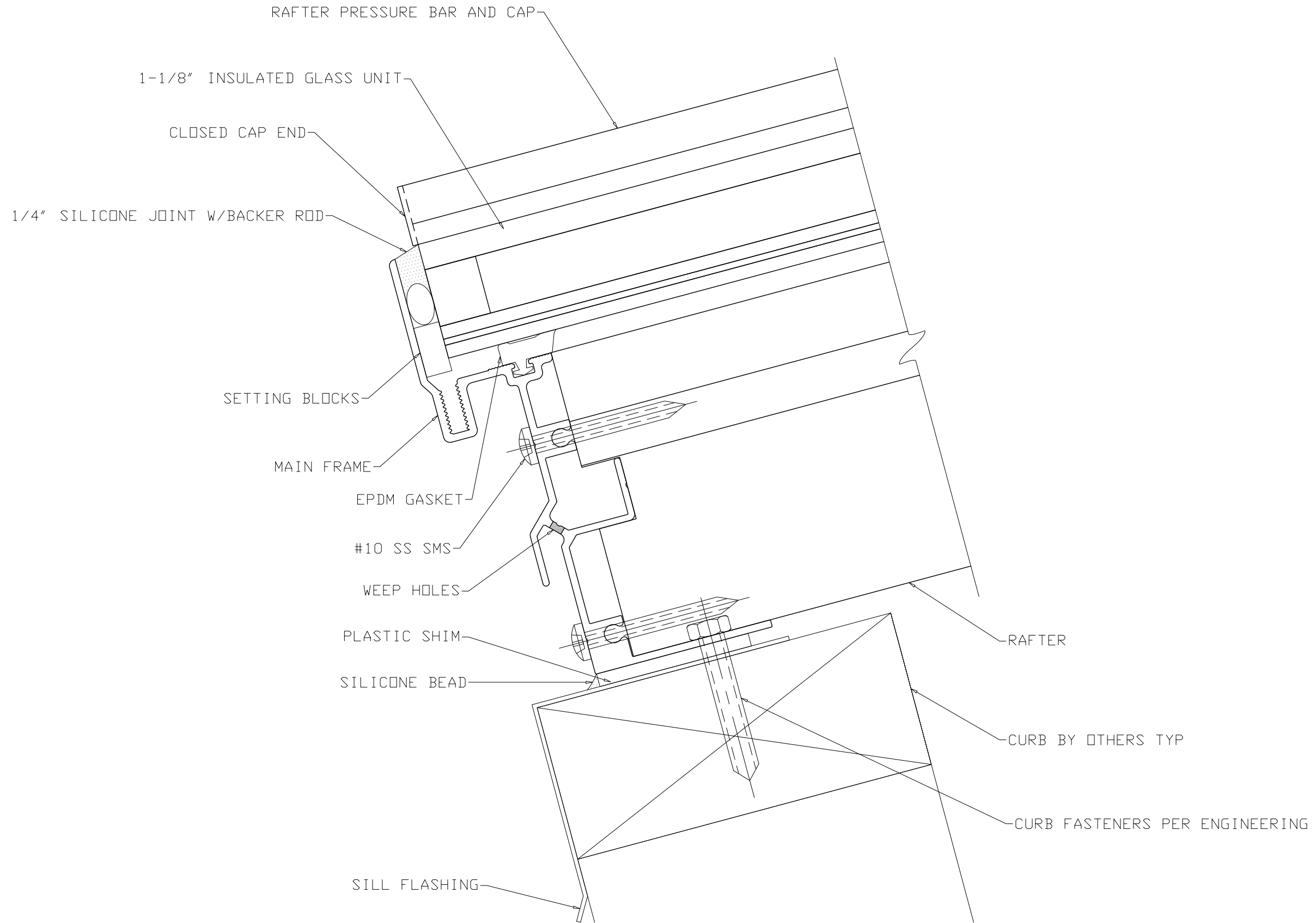
1 SILL SECTION SCALE 1' - 0" = 1' - 0"
