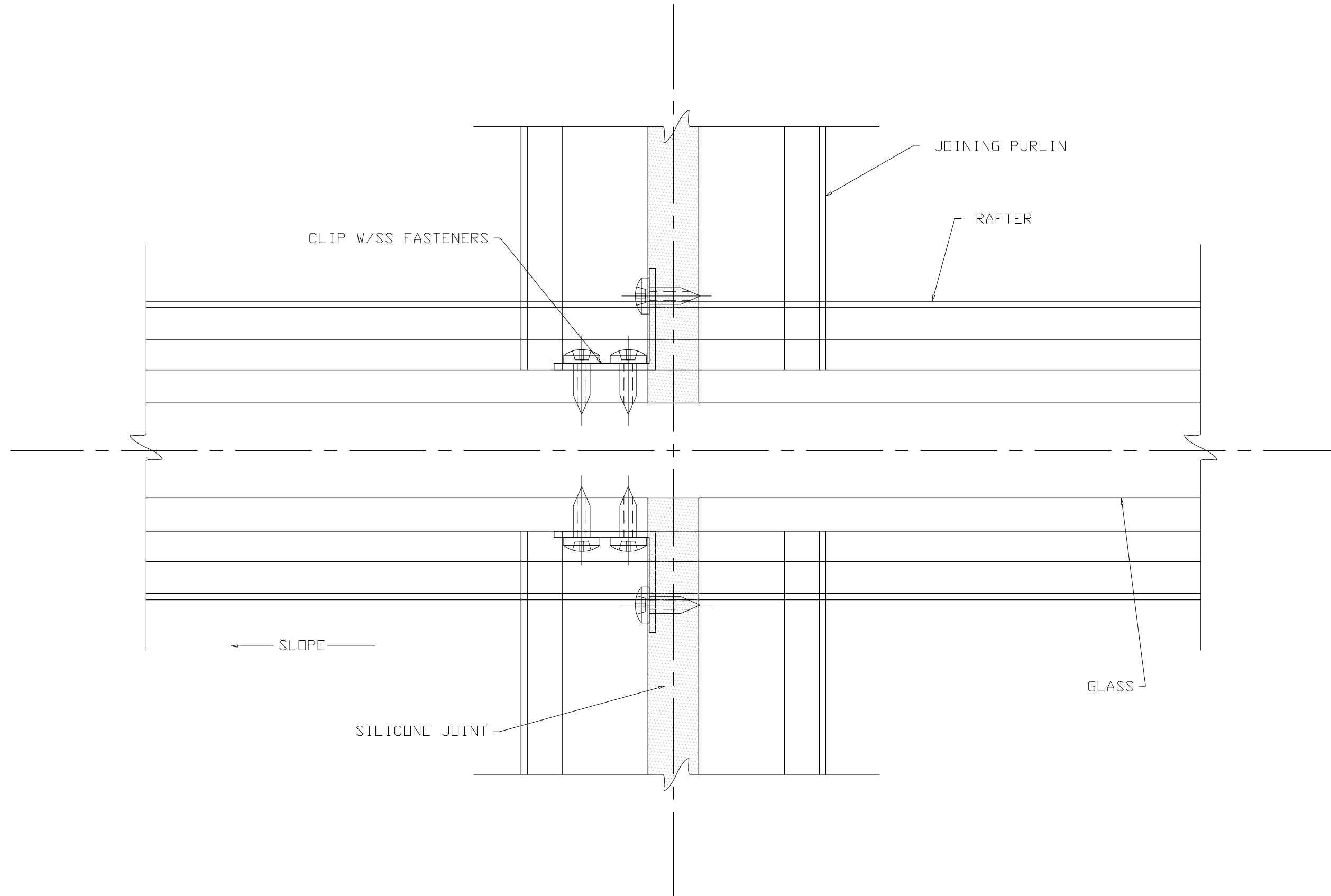
4 PURLIN DETAIL SCALE 1' - 0" = 1' - 0"
