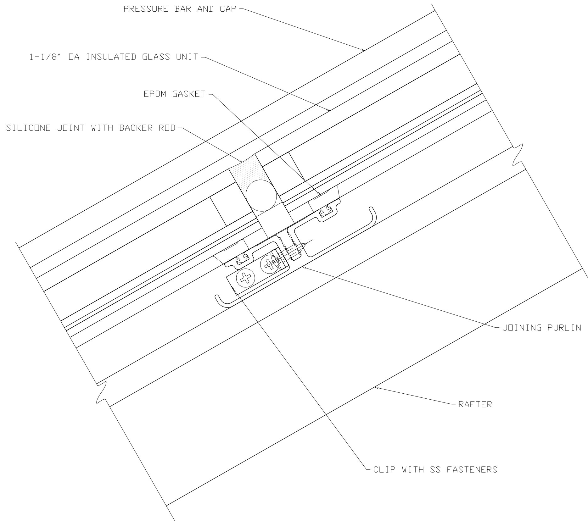
2 PURLIN SECTION SCALE 1' - 0" = 1' - 0"
