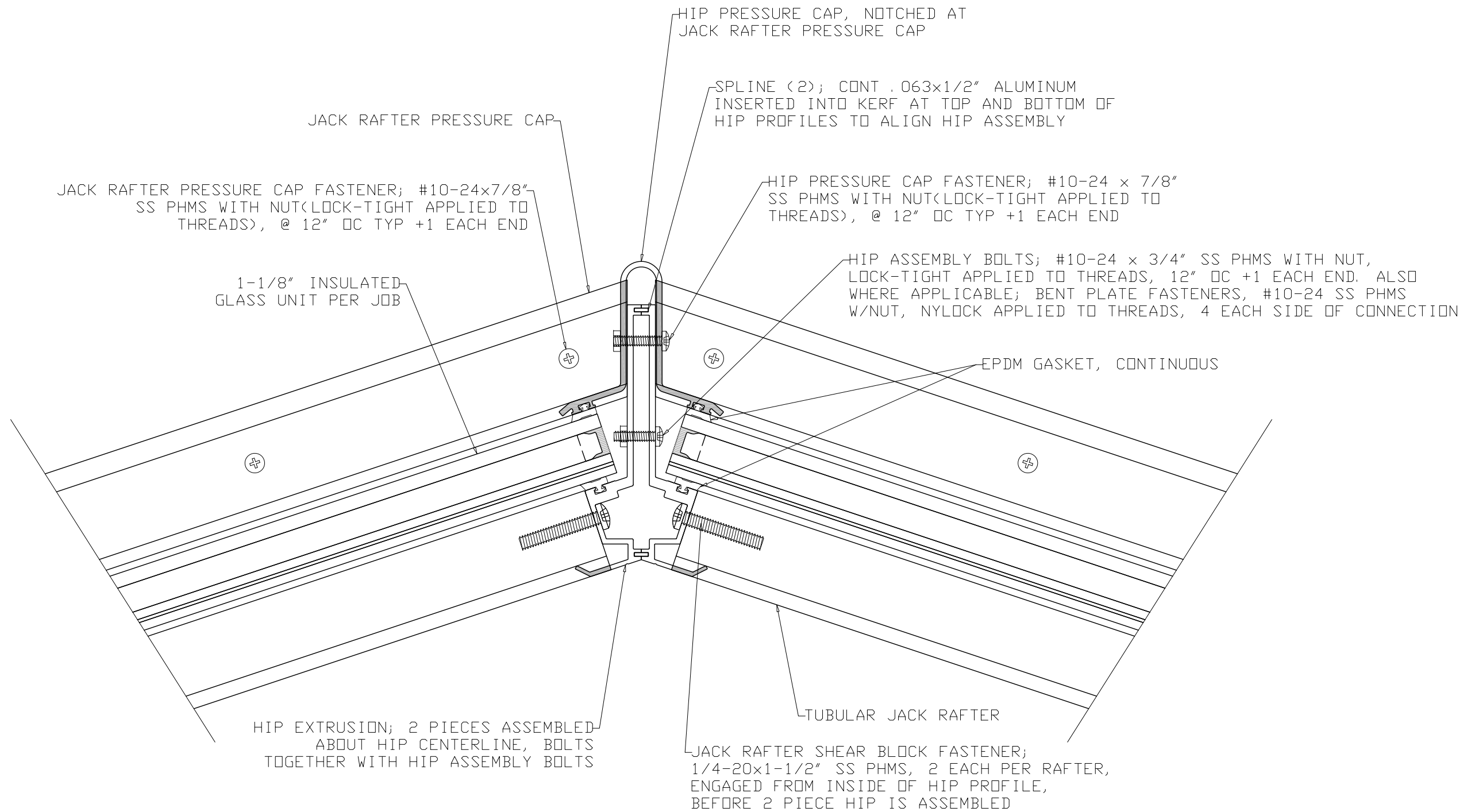
4 HISTORIC HIP DETAIL SCALE 6"=1'-0"
